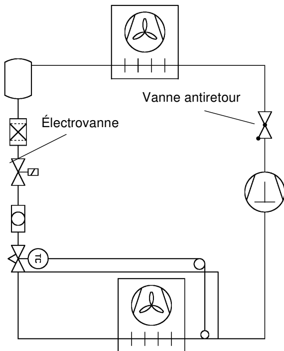
Fig. 6-10. Circuit pump-down
